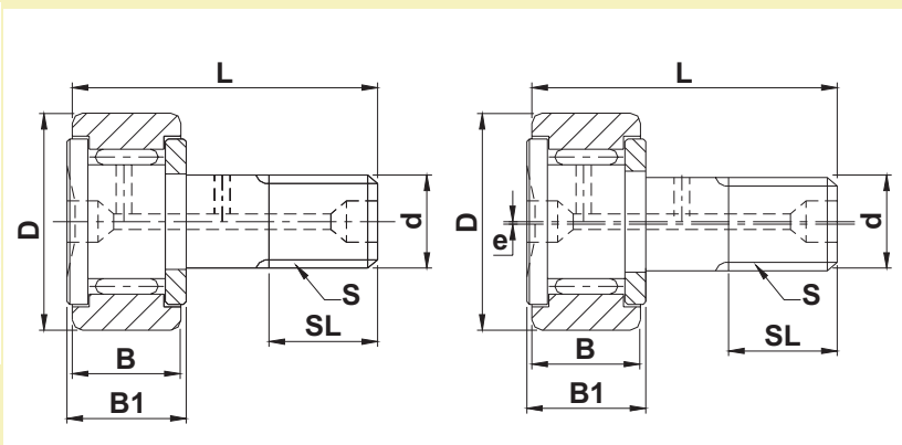
SOLID ECCENTRIC-NCFe
